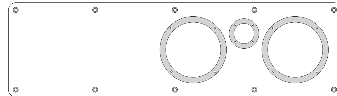
Front Baffle B (Qty: 1)- 3"=1'-0"
